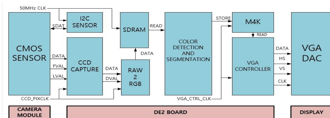
Figure 4: Hardware architecture
