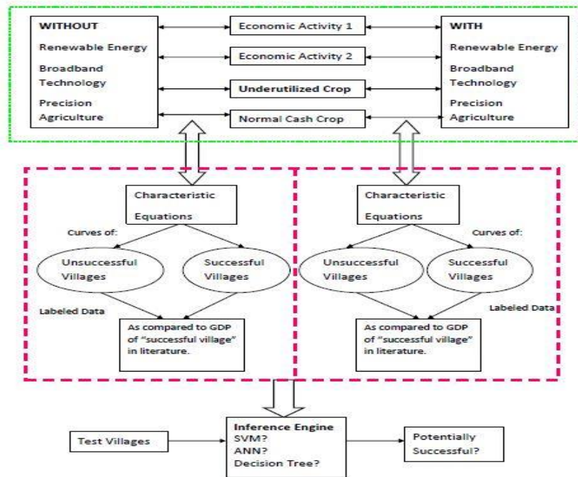
Figure 1: System Architecture
