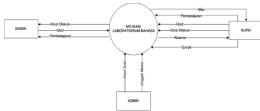
Figure 6: DFD Context Diagram
