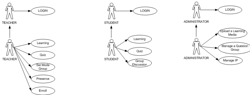
Figure 4: Use Case Diagram
